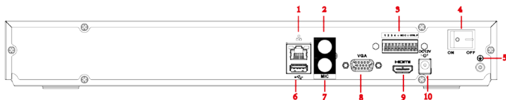
Figura 2-68 Panel trasero
