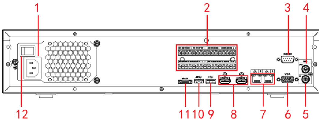
Figura 2-74 Panel trasero
