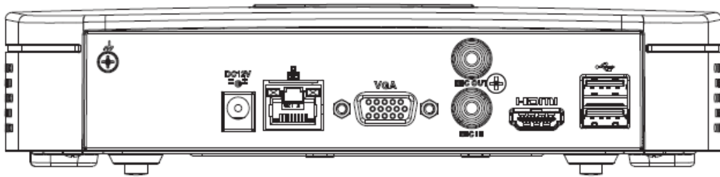
Figura 2-25 Panel trasero
