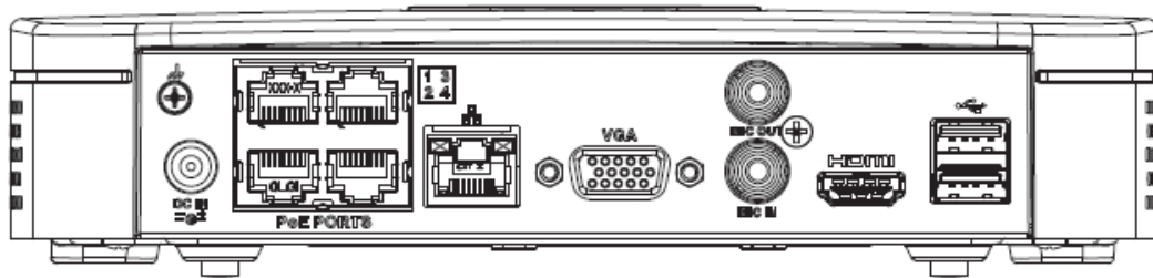
Figura 2-26 Panel trasero
