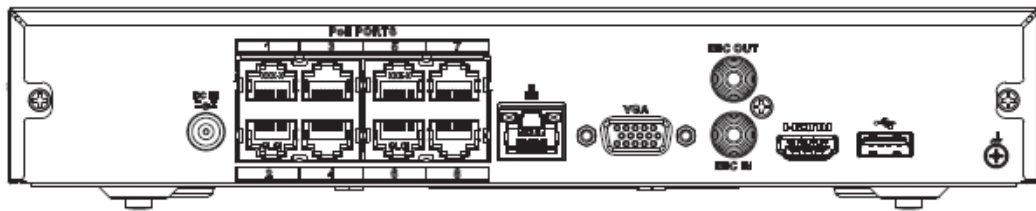
Figura 2-30 Panel trasero
