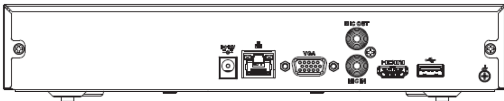
Figura 2-28 Panel trasero
