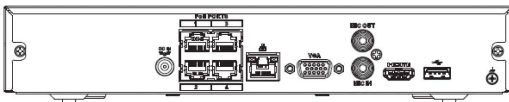
Figura 2-29 Panel trasero
